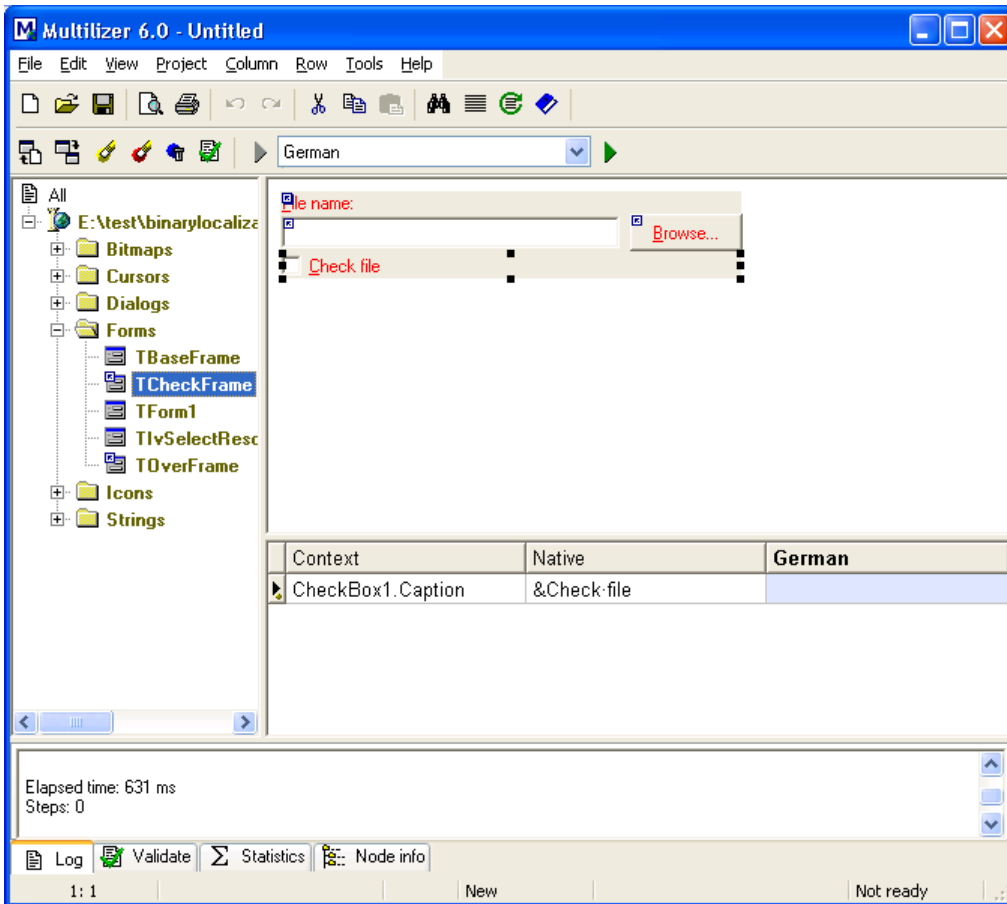
Figure 7: Visual Inheritance: TCheckFrame is an inherited from. Only one string requires translation as other translations are inherited.
