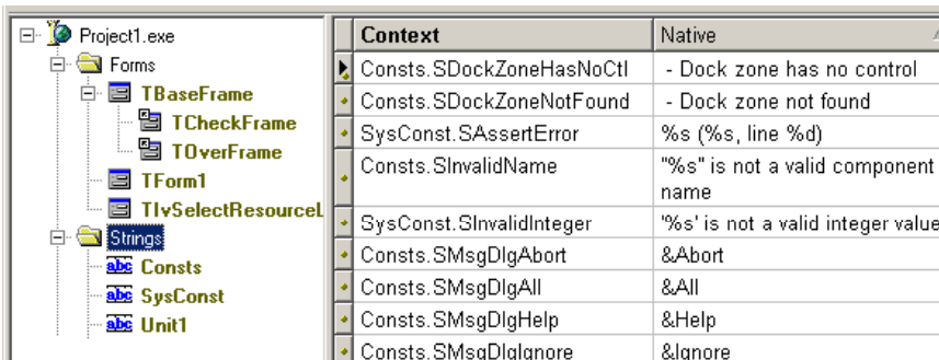
Figure 9: Strings with full context; context is formed out of unit name and resourcestring constant name.
