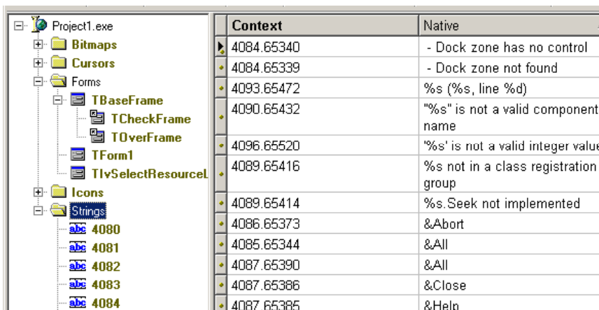
Figure 8: Strings with resource id's as context; Delphi compiler creates the id's, and on each compilation resourcestrings may get different id's.
